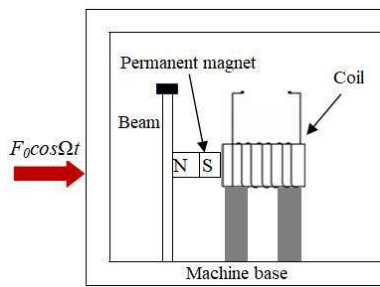
Figure 2. Energy-harvesting model using a linear generator
