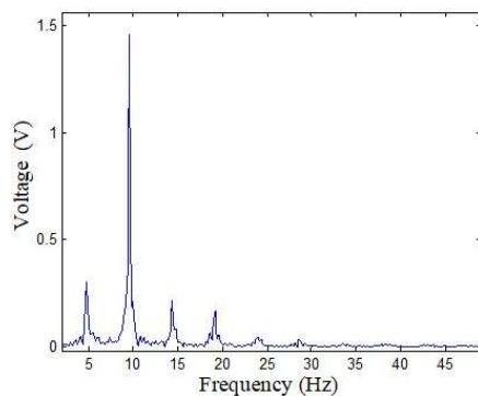
b. Spectrum of the output load voltage
