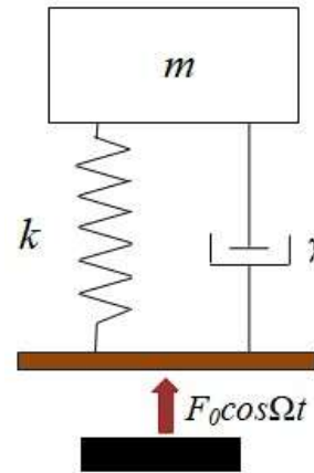
Figure 3. Mechanical model of the device
