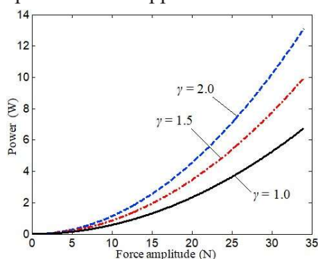
Figure 7. The graph of mechanical power versus the amplitude of the applied external force
