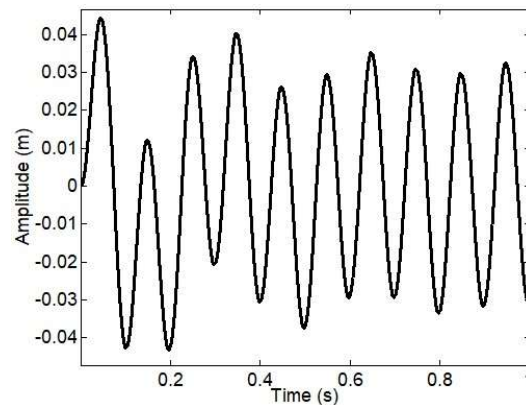
Figure 5. The oscillation of the model versus time
