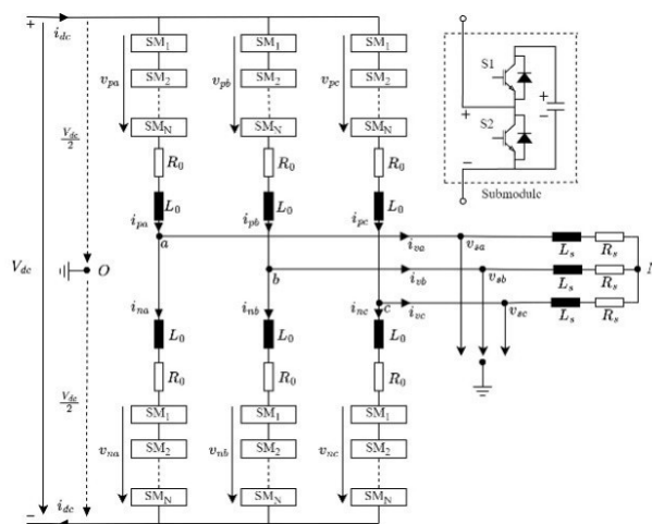
Figure 1. MMC topology
