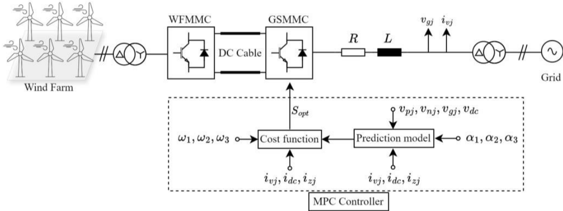
Figure 2. Proposed control scheme
