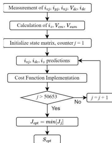
Figure 3. MPC control algorithm
