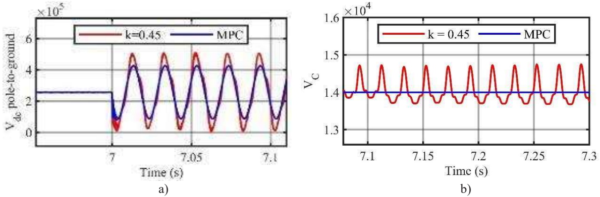
Figure 5. Comparison between zero-sequence method and MPC-based method
