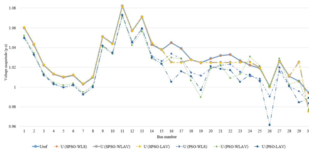
Figure 7. The estimated voltage magnitude in IEEE 30-bus – Case 1
