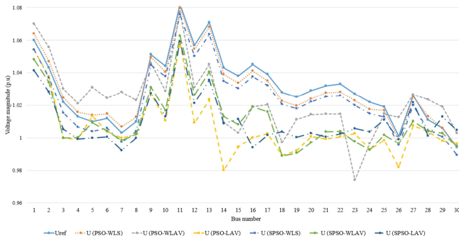
Figure 4. The estimated voltage magnitude in IEEE 14-bus – Case 2
