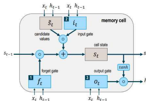
Figure 2. Internal structure of an LSTM cell
