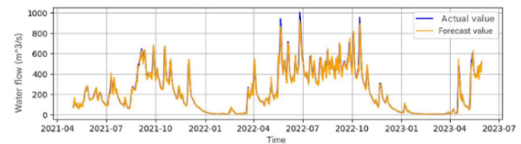
Figure 6. Ten-Step Forecasting Results on the Test Set Using the CNN-LSTM Model
