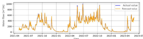
Figure 5. One-Step Forecasting Results on the Test Set Using the CNN-LSTM Model
