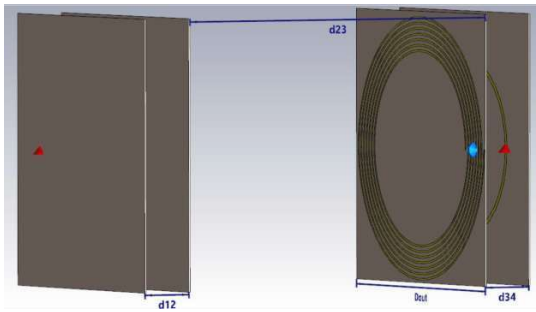
Figure 4. The design model of the MR-WPT system
