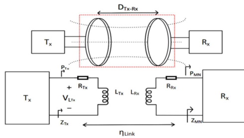
Figure 1. The schematic of the two-coil WPT system.
