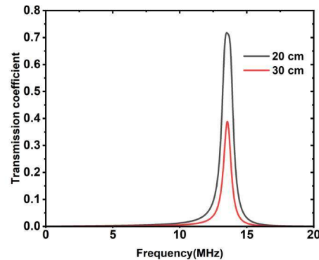
Figure 6. The transfer coefficient of four-coil WPT system
