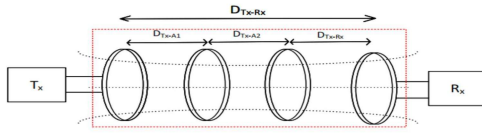
Figure 3. The schematic of four-coil WPT system
