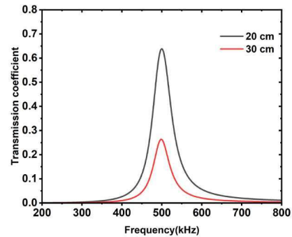
Figure 5. The transfer coefficient of two-coil system
