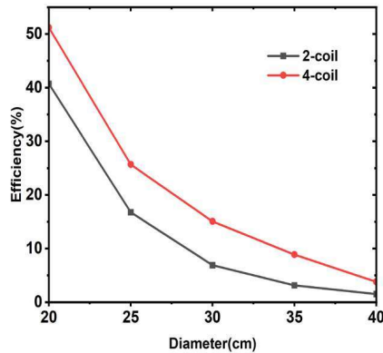
Figure 7. Comparison of Efficiency between the two-coil system and the four-coil system
