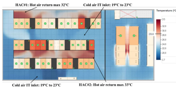
Figure 7. Top view - Cold and Hot air distribution in the IT room (simulated results with actual parameters of Inrow: return air temperature and airflow supply)
