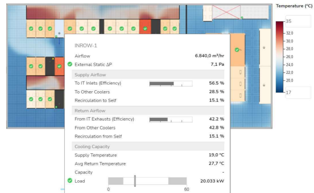
Figure 9. Inrow cooling capacity (simulated results with actual parameters: return air temperature and airflow supply)
