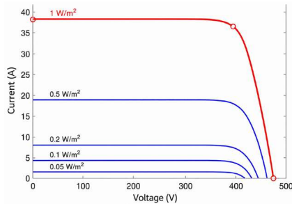
Figure 2. U-I characteristic of the rooftop solar power system at 25°C
