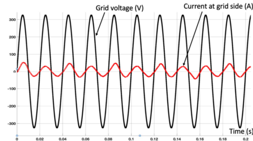
Figure 7. Grid voltage and current at grid side at 400 W/m 2 , 25°C
