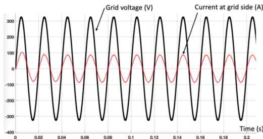
Figure 6. Grid voltage and current at grid side at 1000 W/m 2 , 25°C
