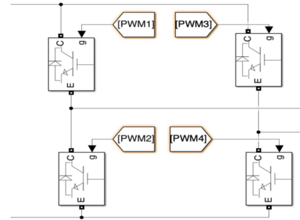
Figure 4. Structure of DC/AC inverter using IGBT/Diode controlled by PWM
