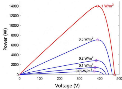
Figure 3. The P-V characteristic of the rooftop solar power system at 25°C
