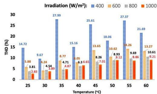
Figure 8. THD of grid side current as a function of temperature and irradiance
