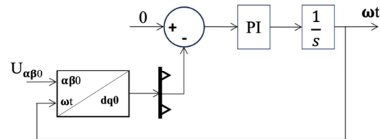
Figure 5. Block diagram of the Phase Locked Loop
